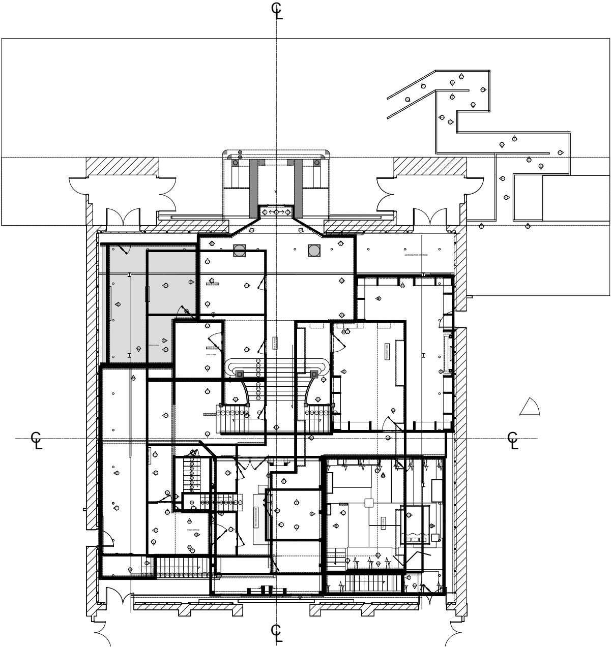
1 WALL THREE GPI Scale: 1/4" = 1'-0"
