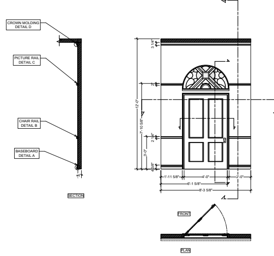
SH7 [SERVANT HALL WALL ELEVATION] Scale: 1/2" = 1'-0"
