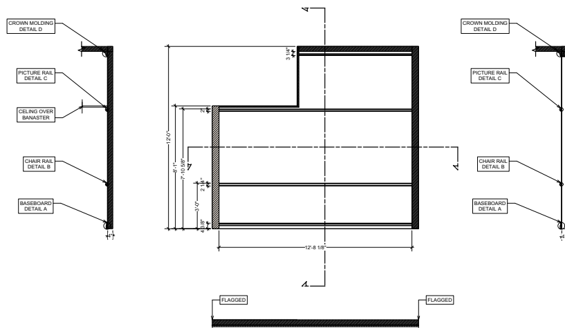
SH3 [SERVANT HALL WALL ELEVATION] Scale: 1/2" = 1'-0"
