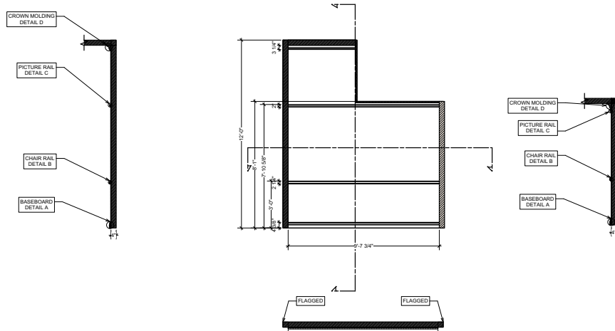
SH1 [SERVANT HALL WALL ELEVATION] Scale: 1/2" = 1'-0"
