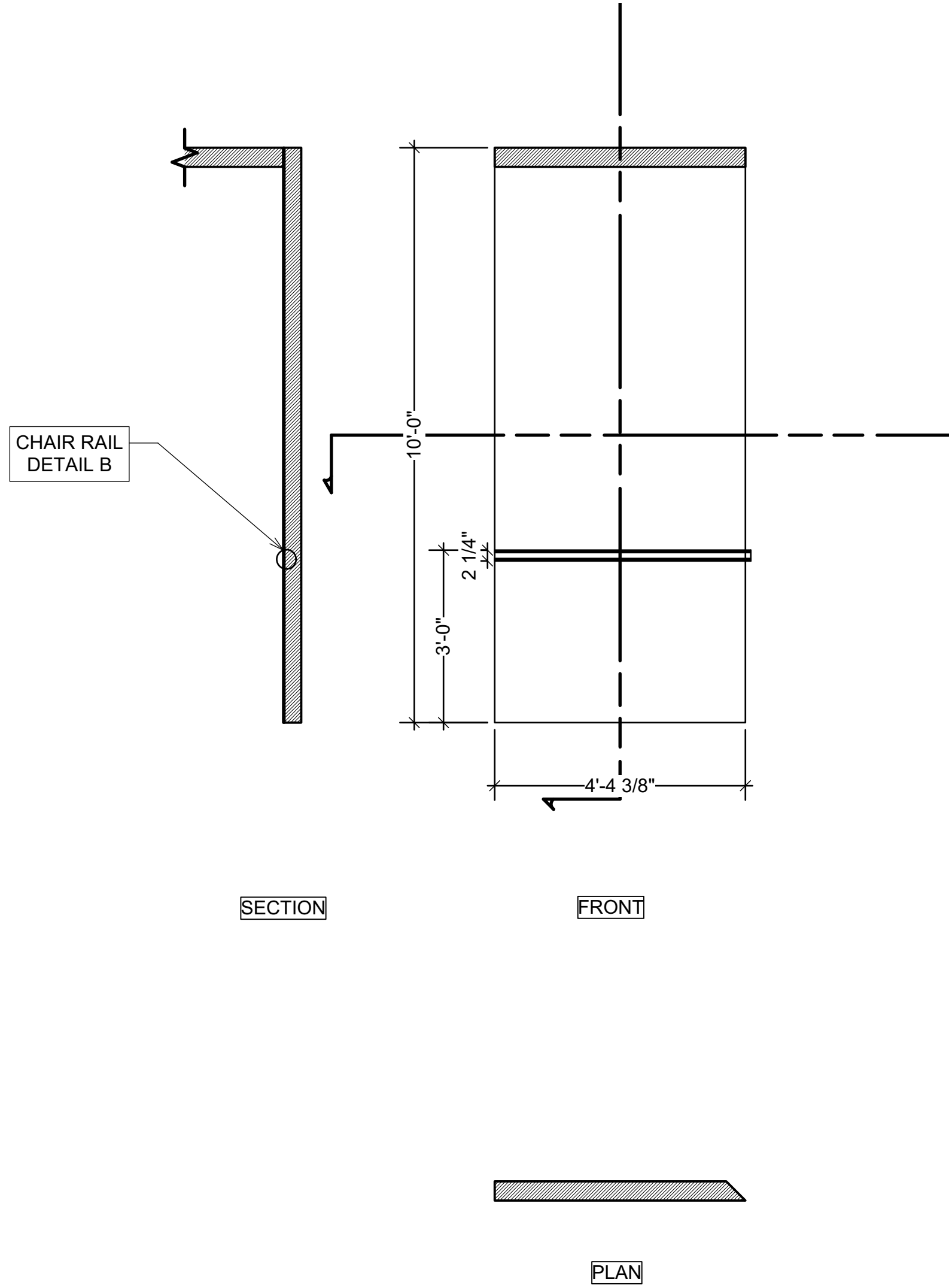
2 [KITCHEN WALL 2] Scale: 1/2\"/>
