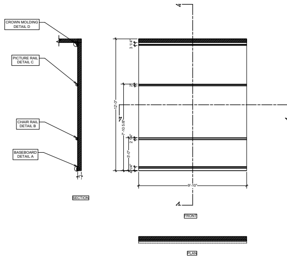
SH8 [SERVANT HALL WALL ELEVATION] Scale: 1/2" = 1'-0"
