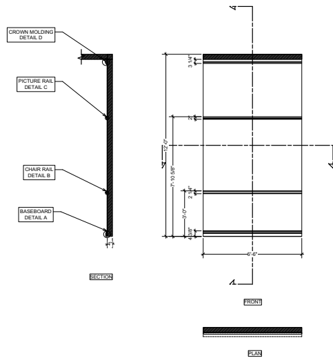
SH6 [SERVANT HALL WALL ELEVATION] Scale: 1/2" = 1'-0"
