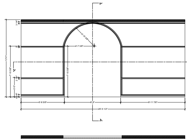
SH4 [SERVANT HALL WALL ELEVATION] Scale: 1/2" = 1'-0"
