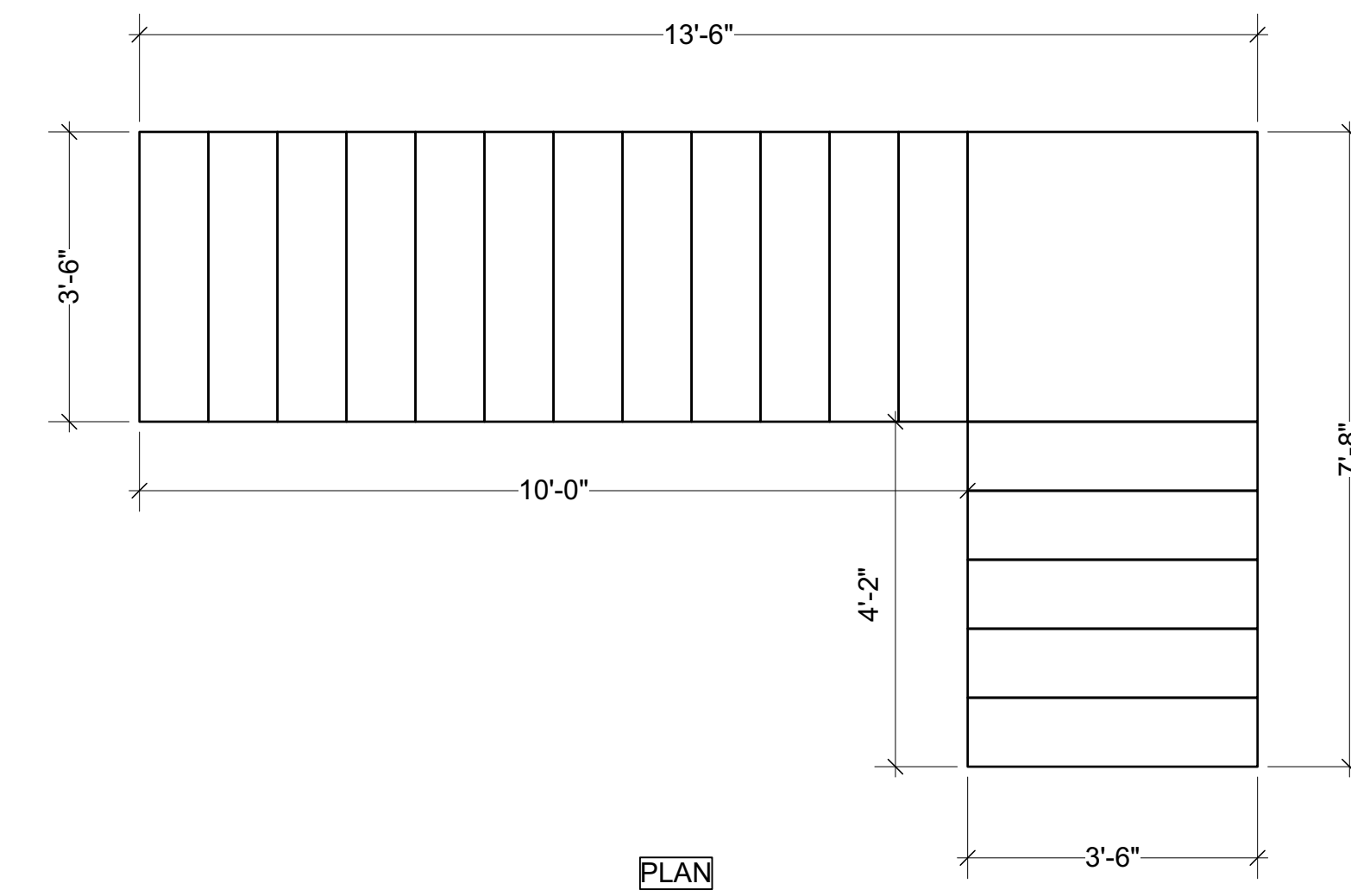
LS [LEDA STAIRCASE] Scale: 1/2" = 1'-0"
