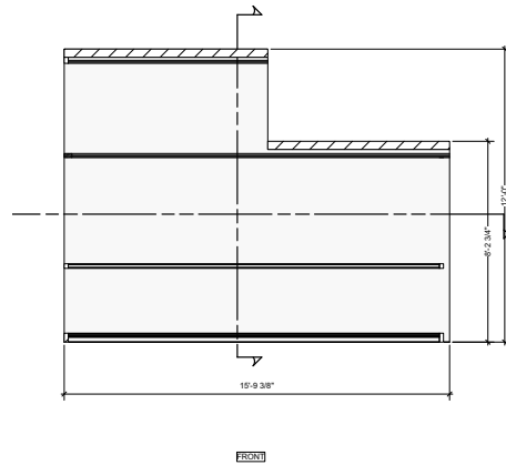
A8 [ATRIUM WALL ELEVATION] Scale: 1/2" = 1'-0"
