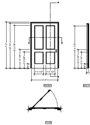
SH7 DO [SH7 DOOR DETAIL] Scale: 1/2" = 1'-0"
