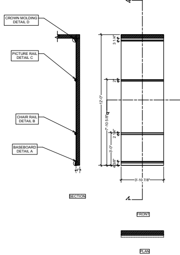
SH9 [SERVANT HALL WALL ELEVATION] Scale: 1/2" = 1'-0"
