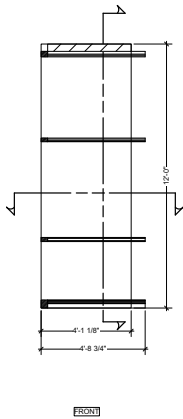
A7 [ATRIUM WALL ELEVATION] Scale: 1/2" = 1'-0"
